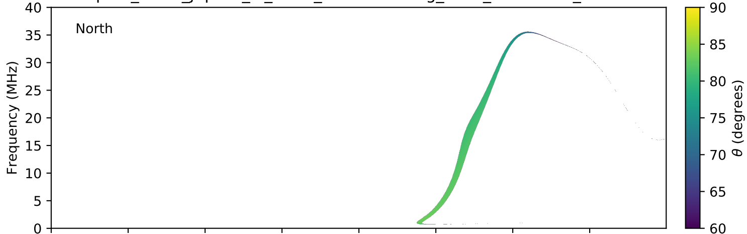
expres_earth_jupiter_io_isaac_lossc-wid1deg_3kev_20050216_v01.cdf
