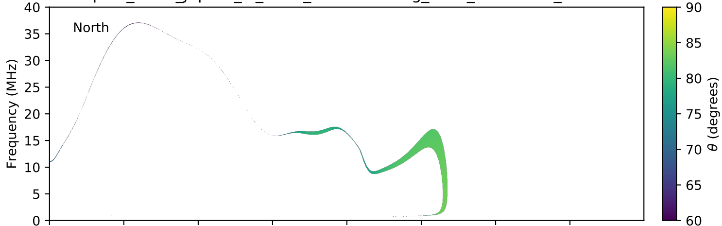
expres_earth_jupiter_io_isaac_lossc-wid1deg_3kev_20050215_v01.cdf
