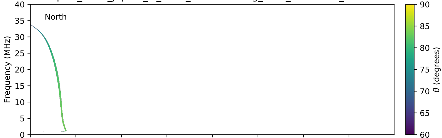
expres_earth_jupiter_io_isaac_lossc-wid1deg_3kev_20050212_v01.cdf
