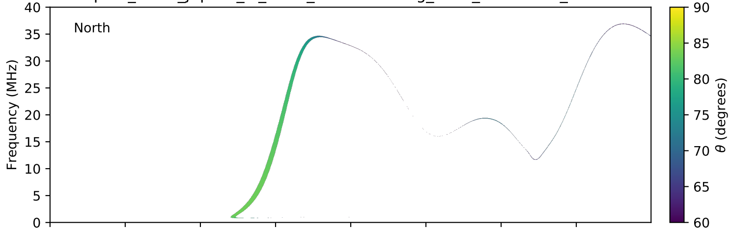
expres_earth_jupiter_io_isaac_lossc-wid1deg_3kev_20050211_v01.cdf
