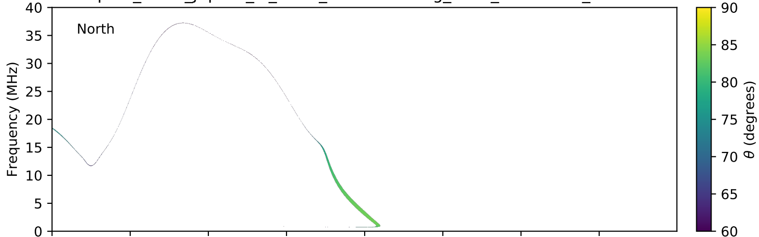
expres_earth_jupiter_io_isaac_lossc-wid1deg_3kev_20050208_v01.cdf
