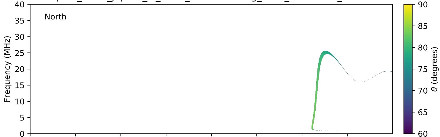
expres_earth_jupiter_io_isaac_lossc-wid1deg_3kev_20050207_v01.cdf
