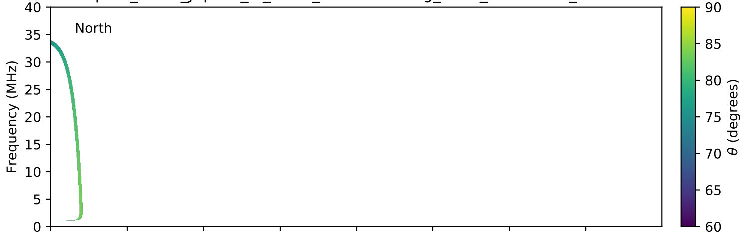
expres_earth_jupiter_io_isaac_lossc-wid1deg_3kev_20050205_v01.cdf
