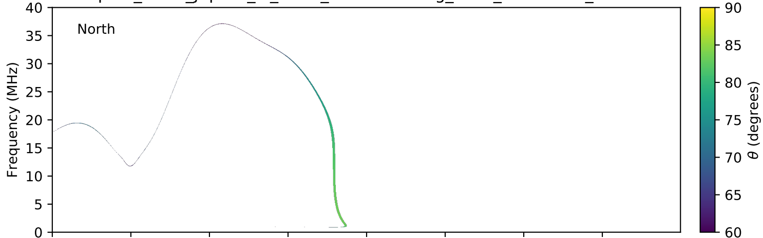
expres_earth_jupiter_io_isaac_lossc-wid1deg_3kev_20050201_v01.cdf
