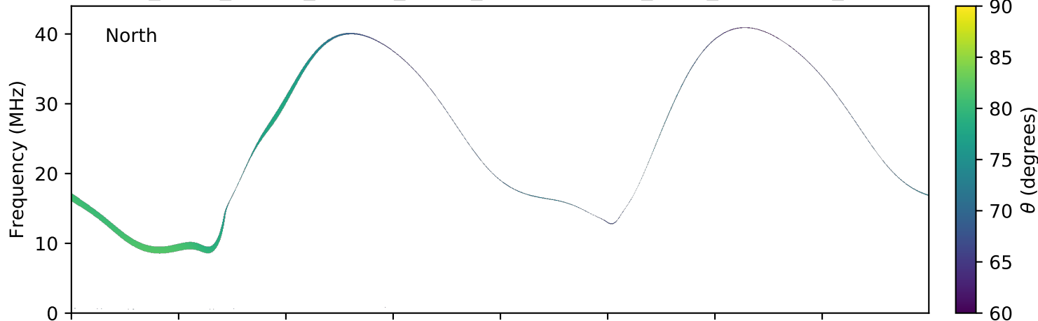
expres_earth_jupiter_europa_jrm09_lossc-wid1deg_3kev_20050223_v01.cdf
