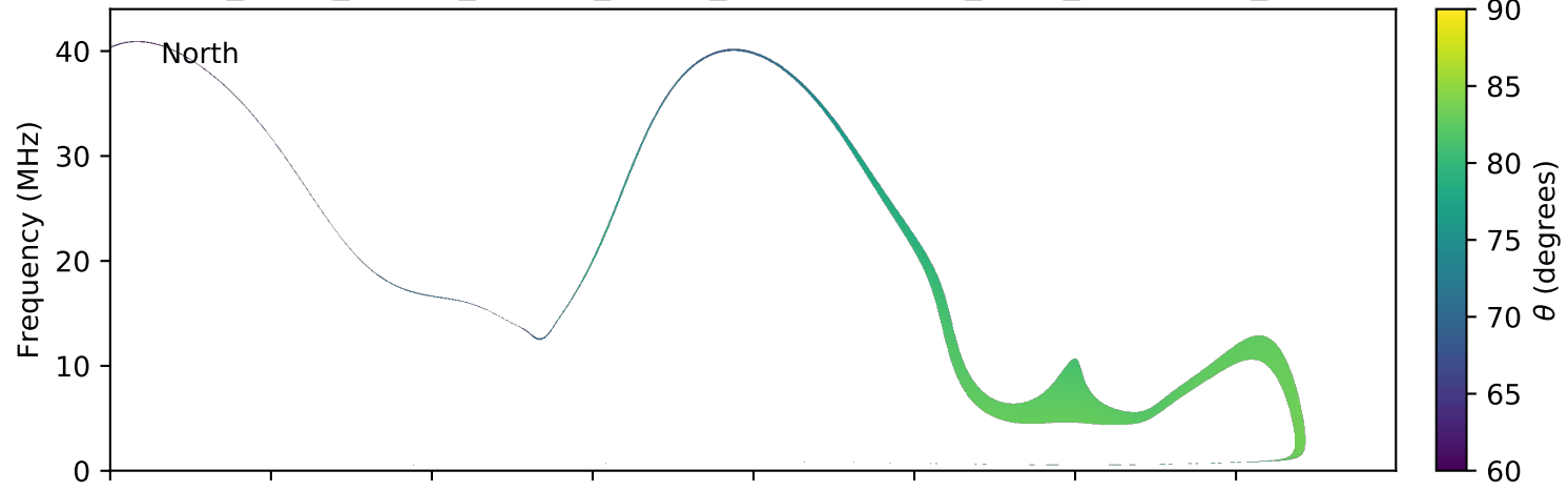
expres_earth_jupiter_europa_jrm09_lossc-wid1deg_3kev_20050213_v01.cdf
