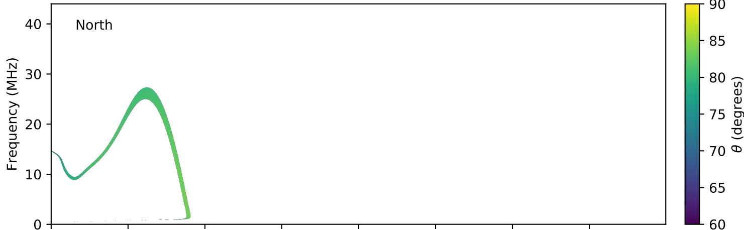
expres_earth_jupiter_europa_jrm09_lossc-wid1deg_3kev_20050203_v01.cdf
