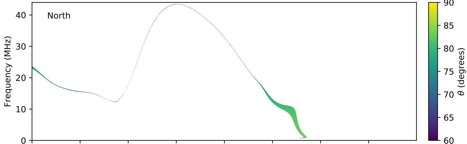
expres_earth_jupiter_io_jrm09_lossc-wid1deg_3kev_20050130_v01.cdf
