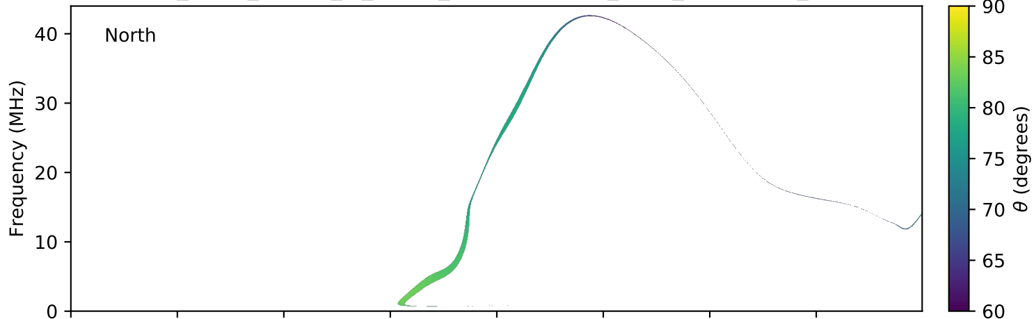
expres_earth_jupiter_io_jrm09_lossc-wid1deg_3kev_20050126_v01.cdf
