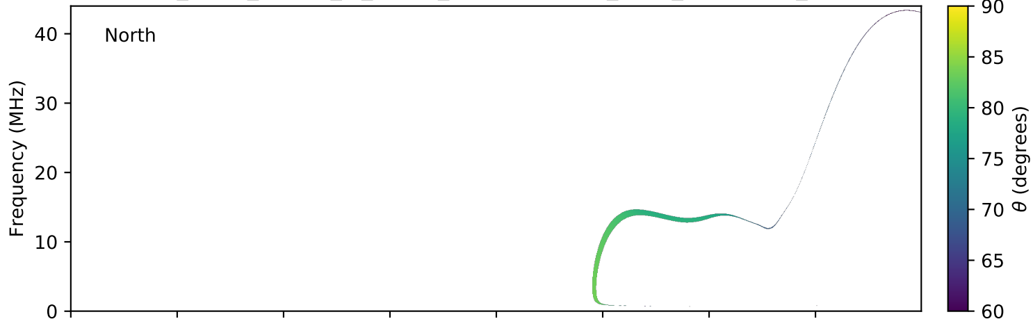
expres_earth_jupiter_io_jrm09_lossc-wid1deg_3kev_20050124_v01.cdf
