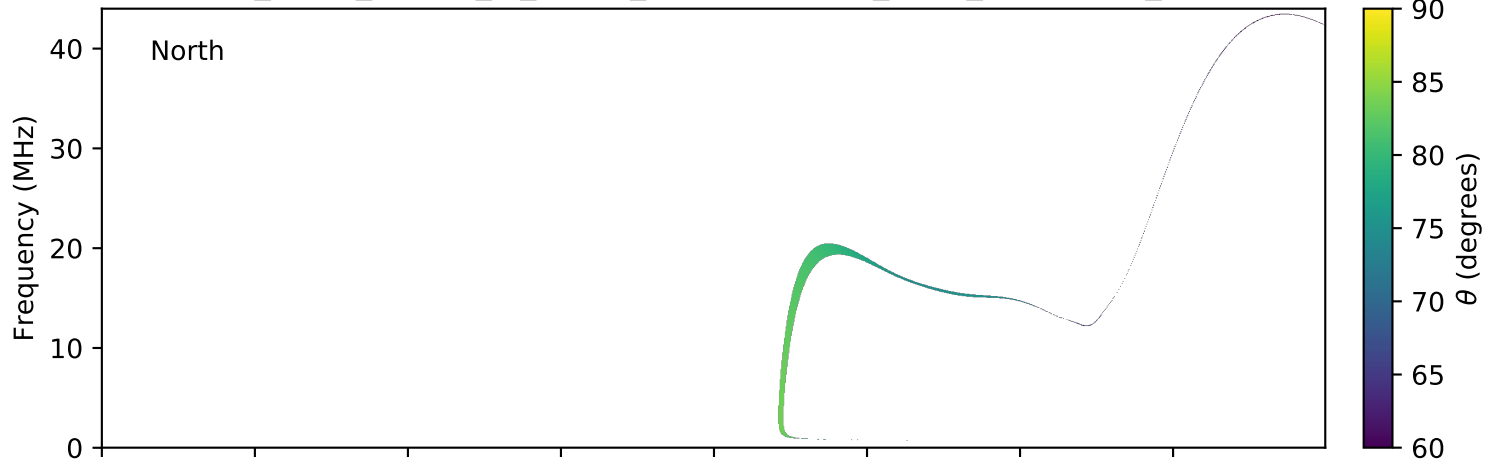
expres_earth_jupiter_io_jrm09_lossc-wid1deg_3kev_20050117_v01.cdf
