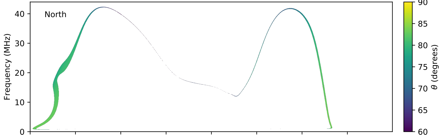
expres_earth_jupiter_io_jrm09_lossc-wid1deg_3kev_20050114_v01.cdf
