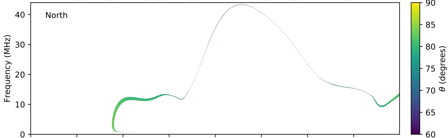
expres_earth_jupiter_io_jrm09_lossc-wid1deg_3kev_20050112_v01.cdf
