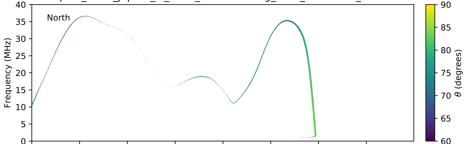
expres_earth_jupiter_io_isaac_lossc-wid1deg_3kev_20050130_v01.cdf
