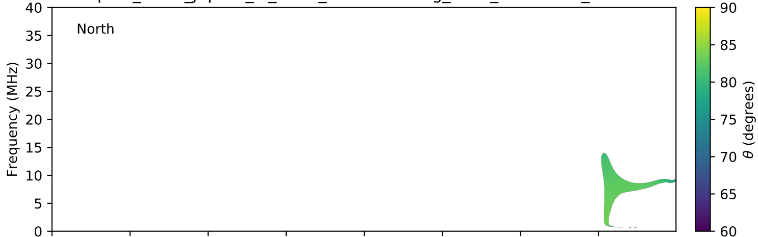
expres_earth_jupiter_io_isaac_lossc-wid1deg_3kev_20050129_v01.cdf
