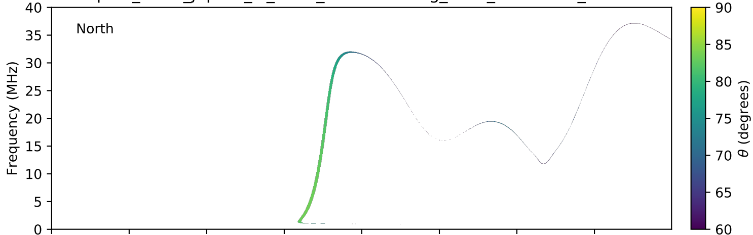
expres_earth_jupiter_io_isaac_lossc-wid1deg_3kev_20050126_v01.cdf
