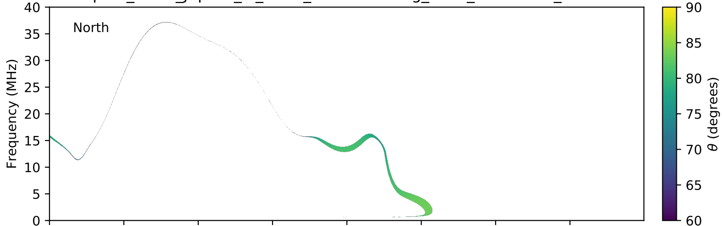
expres_earth_jupiter_io_isaac_lossc-wid1deg_3kev_20050123_v01.cdf
