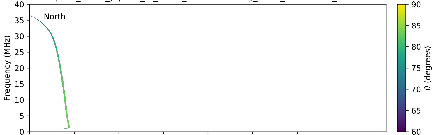
expres_earth_jupiter_io_isaac_lossc-wid1deg_3kev_20050120_v01.cdf
