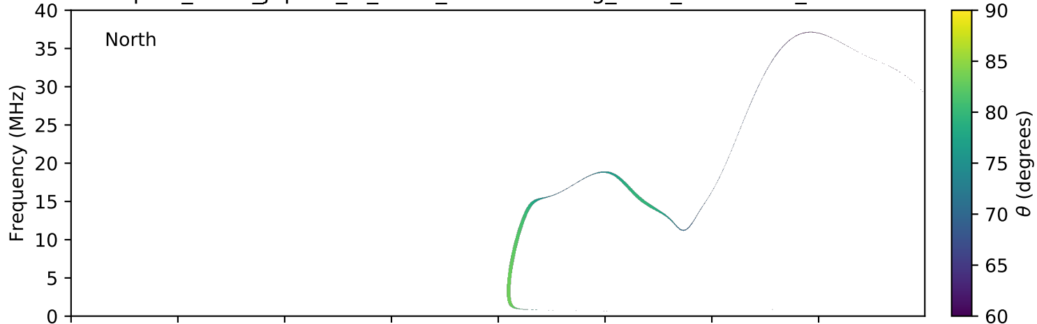
expres_earth_jupiter_io_isaac_lossc-wid1deg_3kev_20050117_v01.cdf
