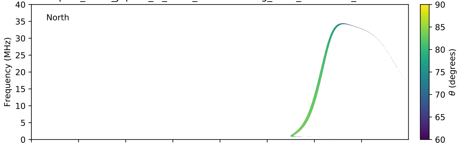
expres_earth_jupiter_io_isaac_lossc-wid1deg_3kev_20050108_v01.cdf
