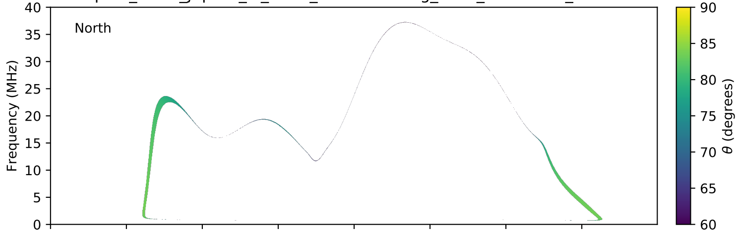
expres_earth_jupiter_io_isaac_lossc-wid1deg_3kev_20050105_v01.cdf
