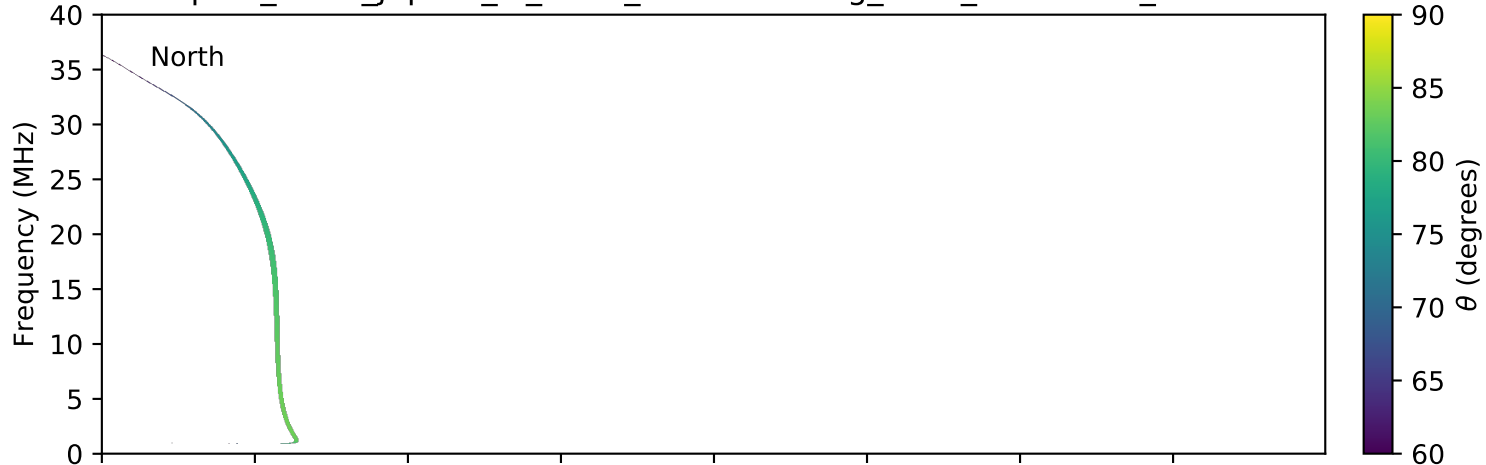
expres_earth_jupiter_io_isaac_lossc-wid1deg_3kev_20050104_v01.cdf
