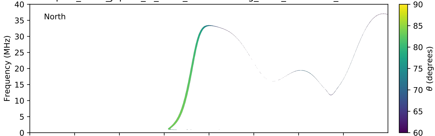
expres_earth_jupiter_io_isaac_lossc-wid1deg_3kev_20050103_v01.cdf
