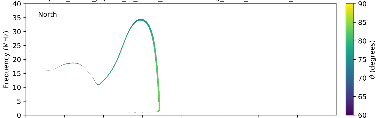
expres_earth_jupiter_io_isaac_lossc-wid1deg_3kev_20050102_v01.cdf
