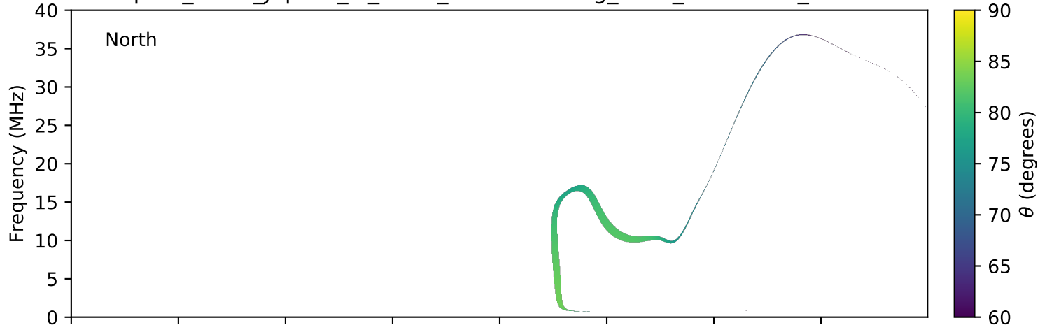
expres_earth_jupiter_io_isaac_lossc-wid1deg_3kev_20050101_v01.cdf
