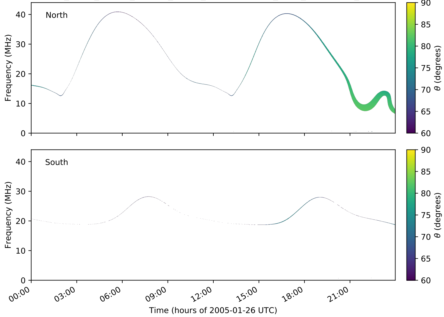
expres_earth_jupiter_europa_jrm09_lossc-wid1deg_3kev_20050126_v01.cdf
