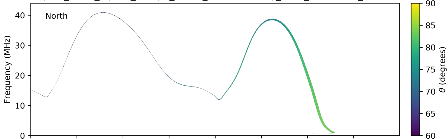
expres_earth_jupiter_europa_jrm09_lossc-wid1deg_3kev_20050112_v01.cdf
