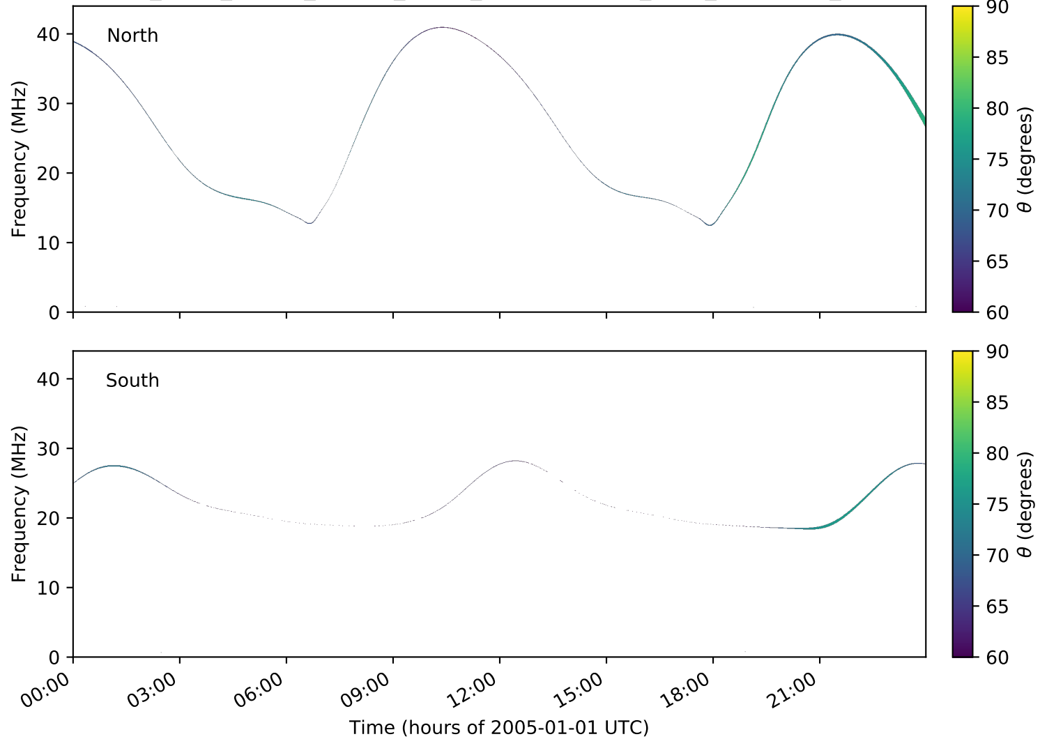
expres_earth_jupiter_europa_jrm09_lossc-wid1deg_3kev_20050101_v01.cdf
