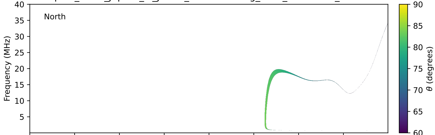
expres_earth_jupiter_io_jrm33_lossc-wid1deg_3kev_20031221_v11.cdf
