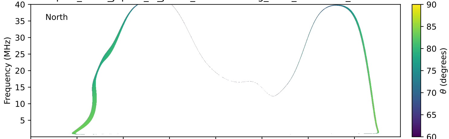
expres_earth_jupiter_io_jrm33_lossc-wid1deg_3kev_20031218_v11.cdf
