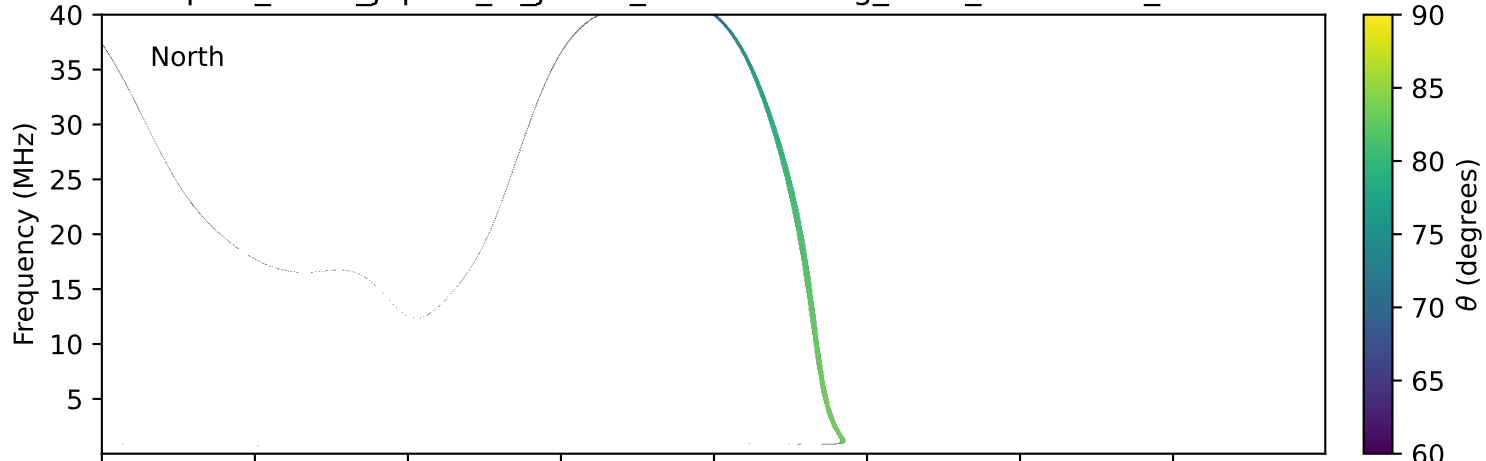
expres_earth_jupiter_io_jrm33_lossc-wid1deg_3kev_20031213_v11.cdf
