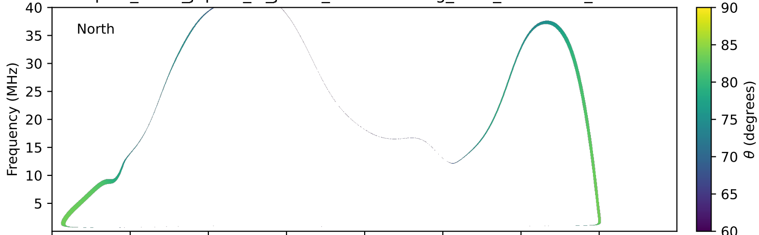
expres_earth_jupiter_io_jrm33_lossc-wid1deg_3kev_20031211_v11.cdf
