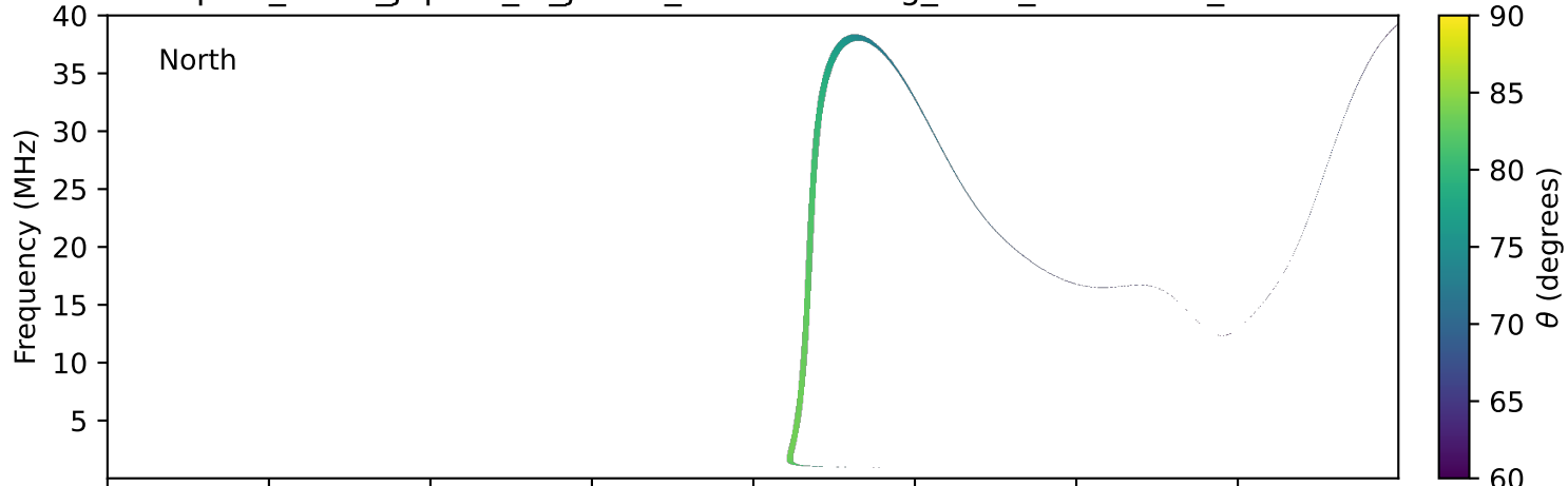
expres_earth_jupiter_io_jrm33_lossc-wid1deg_3kev_20031207_v11.cdf
