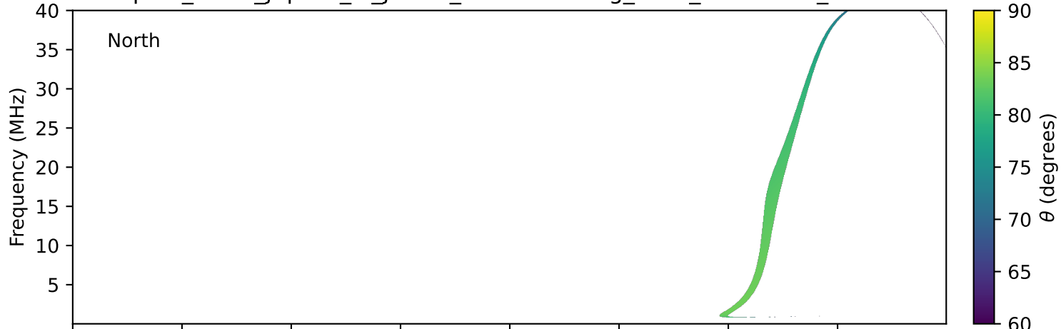
expres_earth_jupiter_io_jrm33_lossc-wid1deg_3kev_20031205_v11.cdf
