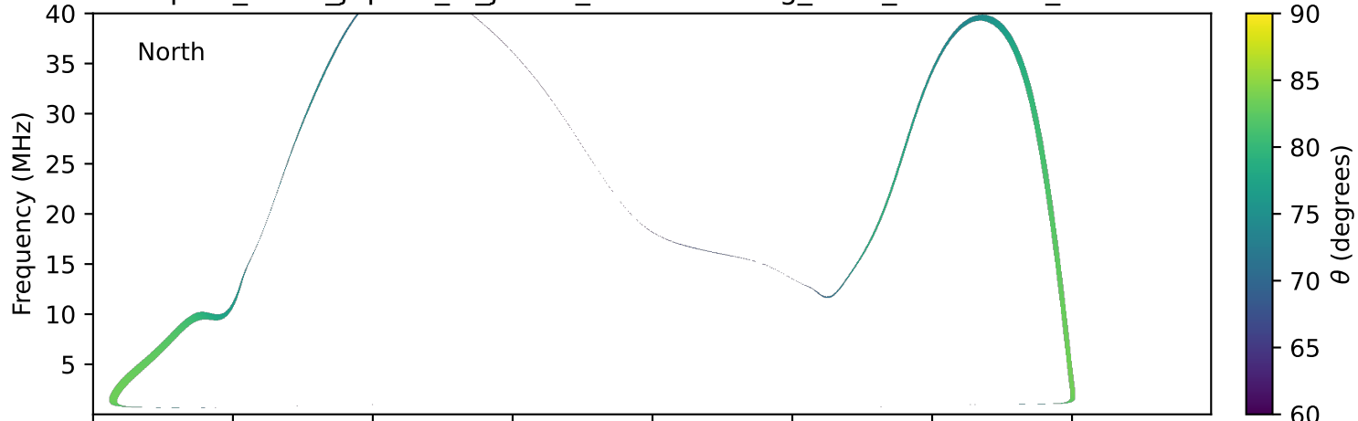
expres_earth_jupiter_io_jrm09_lossc-wid1deg_3kev_20031211_v11.cdf
