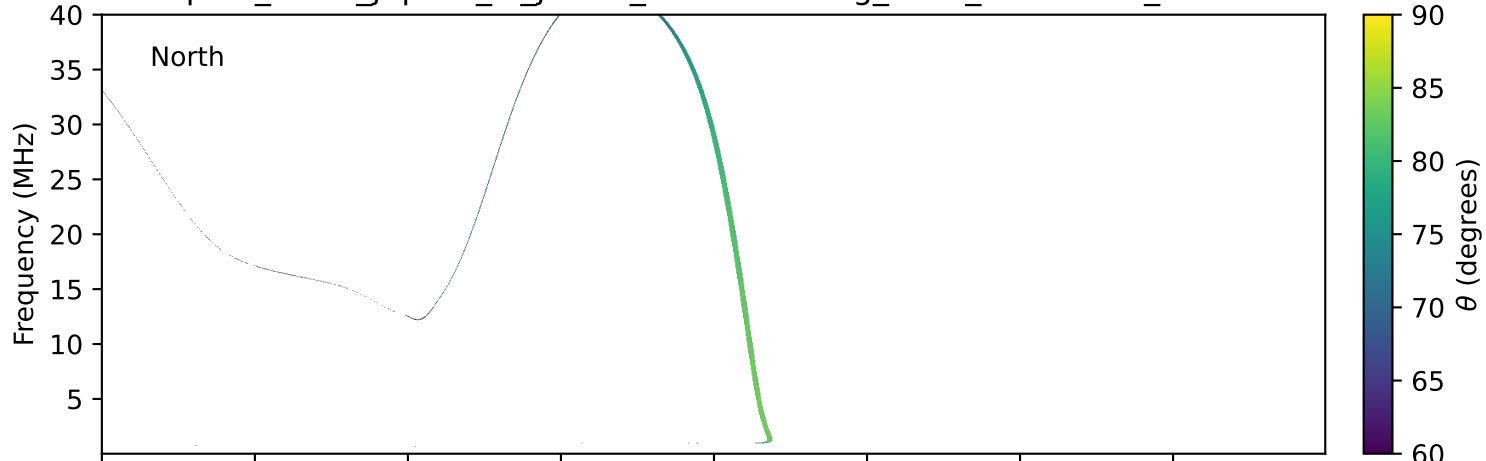
expres_earth_jupiter_io_jrm09_lossc-wid1deg_3kev_20031206_v11.cdf
