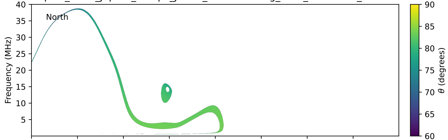
expres_earth_jupiter_europa_jrm33_lossc-wid1deg_3kev_20031215_v11.cdf
