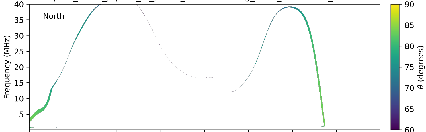
expres_earth_jupiter_io_jrm33_lossc-wid1deg_3kev_20030828_v11.cdf
