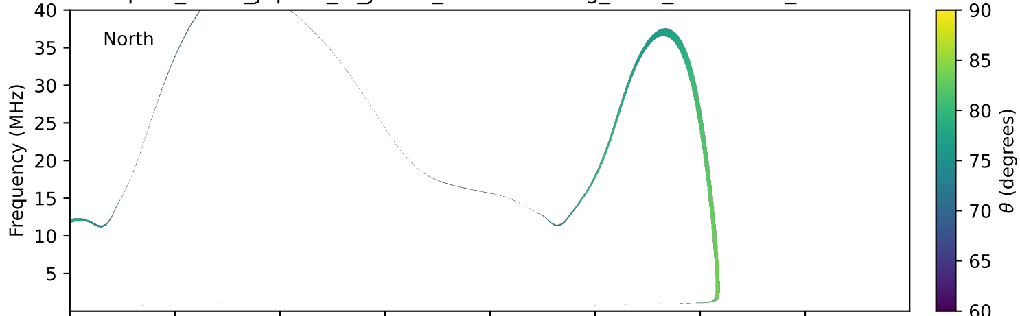
expres_earth_jupiter_io_jrm09_lossc-wid1deg_3kev_20030821_v11.cdf
