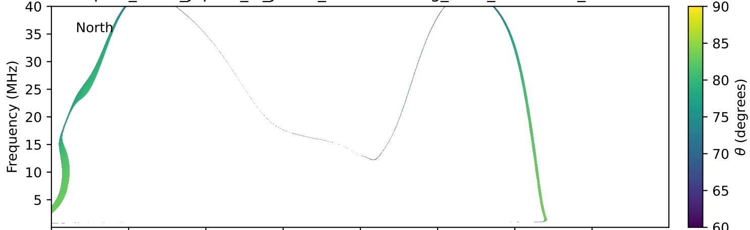
expres_earth_jupiter_io_jrm09_lossc-wid1deg_3kev_20030814_v11.cdf
