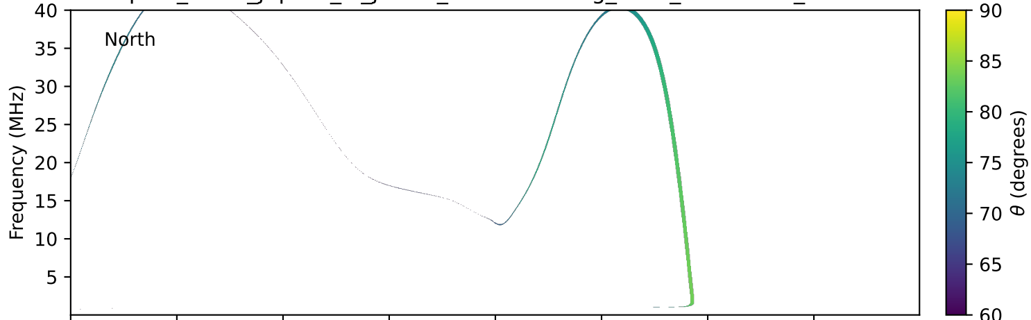
expres_earth_jupiter_io_jrm09_lossc-wid1deg_3kev_20030807_v11.cdf
