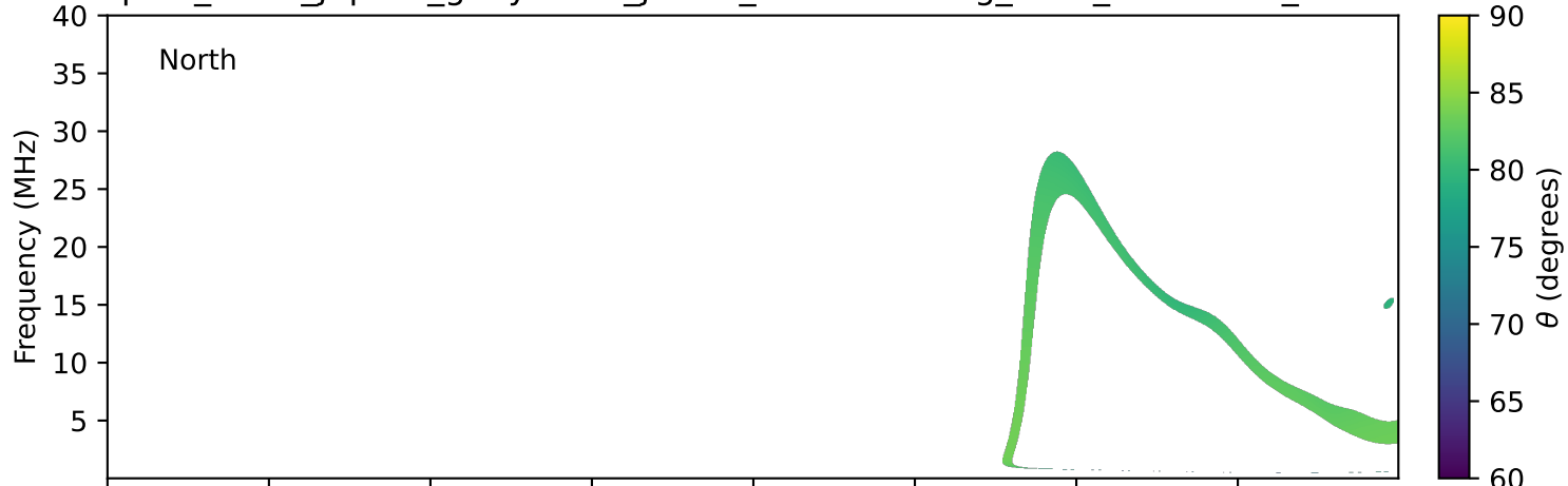
expres_earth_jupiter_ganymede_jrm33_lossc-wid1deg_3kev_20030806_v11.cdf
