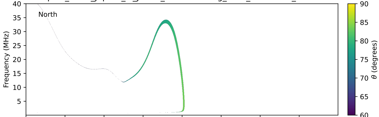
expres_earth_jupiter_io_jrm33_lossc-wid1deg_3kev_20030626_v11.cdf
