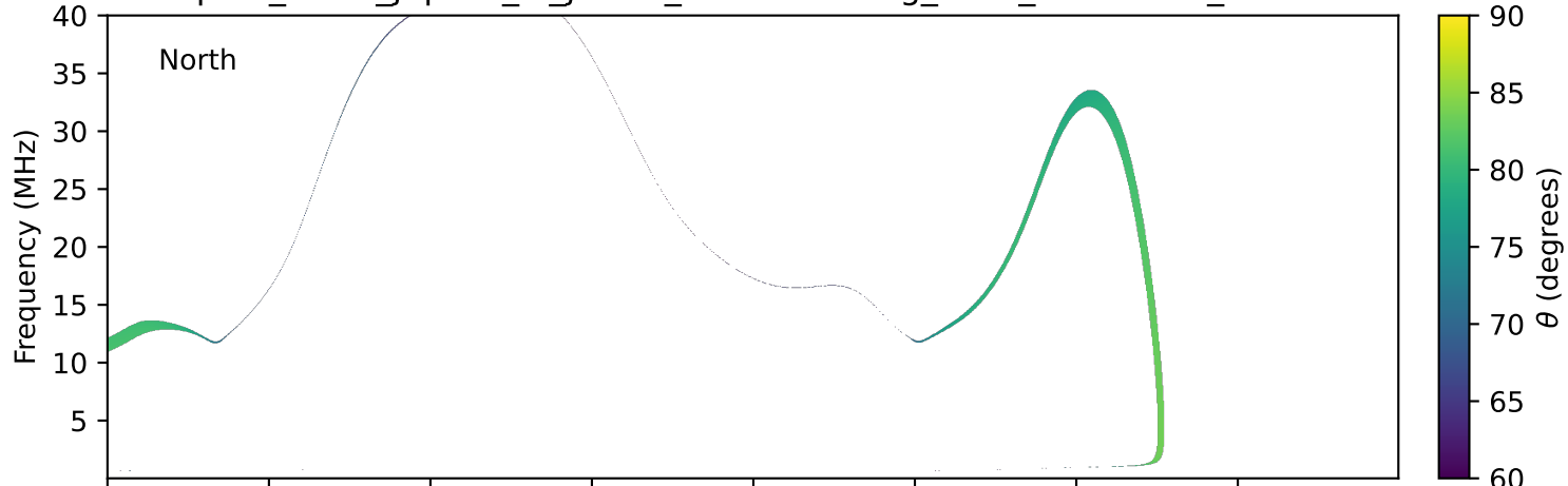
expres_earth_jupiter_io_jrm33_lossc-wid1deg_3kev_20030617_v11.cdf
