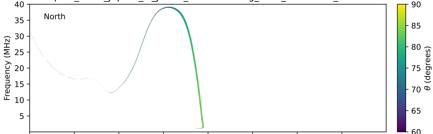
expres_earth_jupiter_io_jrm33_lossc-wid1deg_3kev_20030612_v11.cdf
