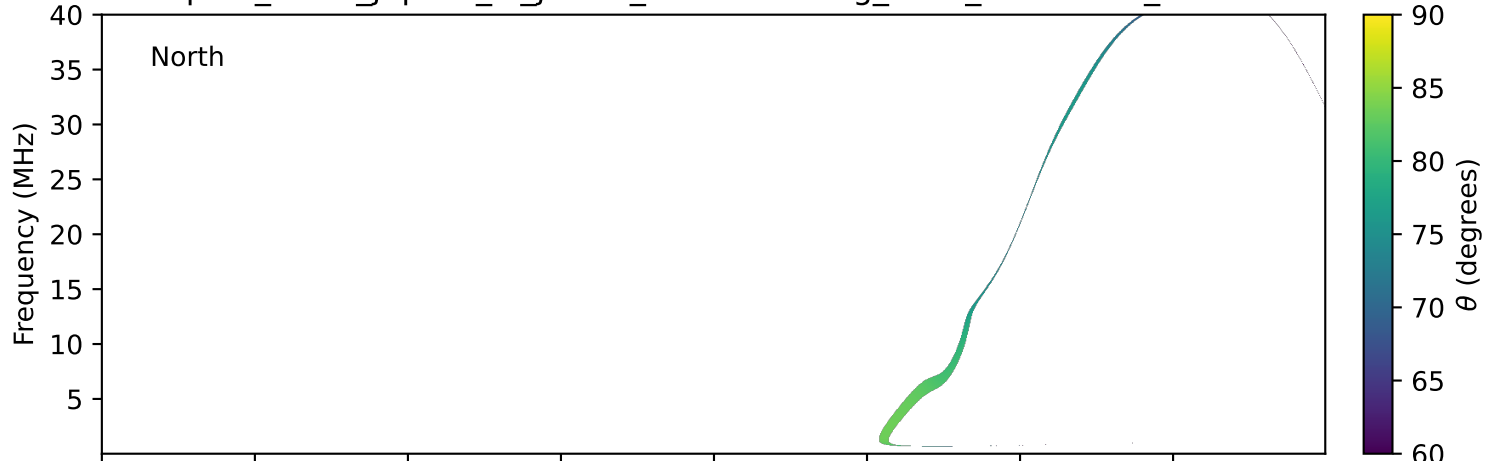
expres_earth_jupiter_io_jrm33_lossc-wid1deg_3kev_20030611_v11.cdf
